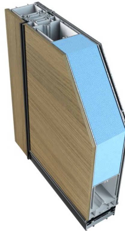
Wood + Aluminium
